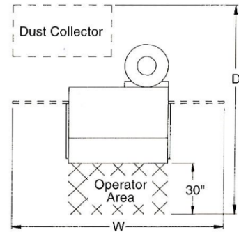
Floor Area Required Shown With 700 CFM Reclaimer
